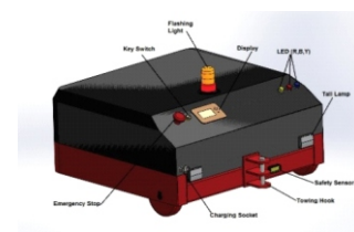
AGV - Auto Guided Vehicle Tow Truck Capacity - 5000 Kgs
